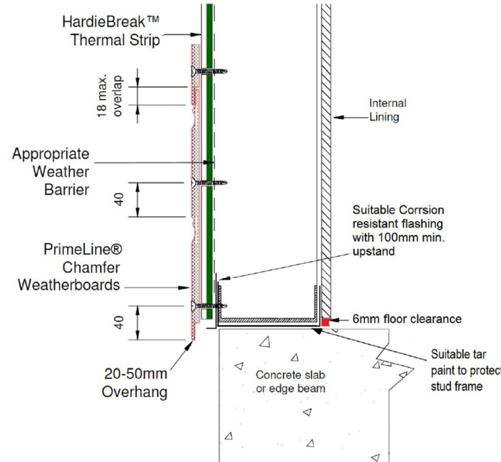
Figure 1: Fixing Detail for Timber Framing in Cyclonic Wind Regions
